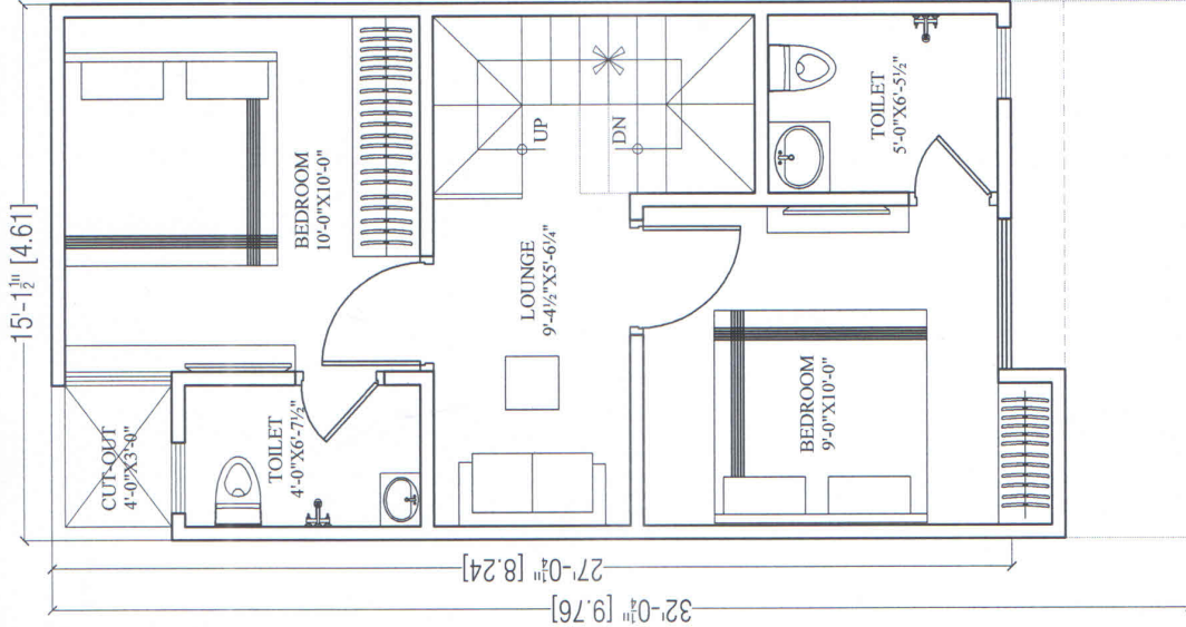
FIRST FLOOR PLAN CARPET AREA = 317.63 SQ. FT. BUILT-UP AREA = 416.68 SQ. FT.
