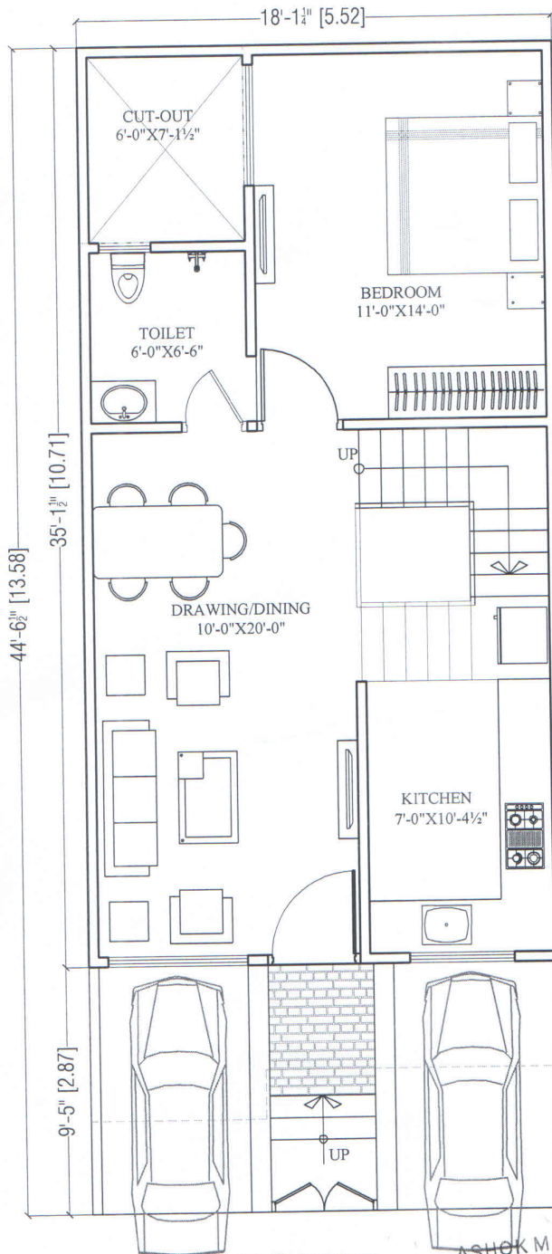
GROUND FLOOR PLAN CARPET AREA = 473.00 SQ.FT. BUILT-UP AREA = 674.00 SQ.FT.
