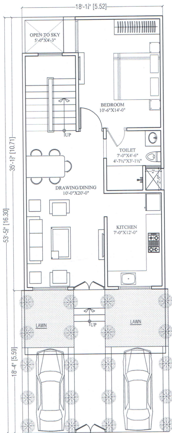
ENTRY GROUND FLOOR PLAN CARPET AREA = 490.00 SQ.FT. BUILT-UP AREA = 755.00 SQ.FT.
